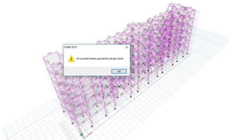
Fig -6: 3D View of Structure
