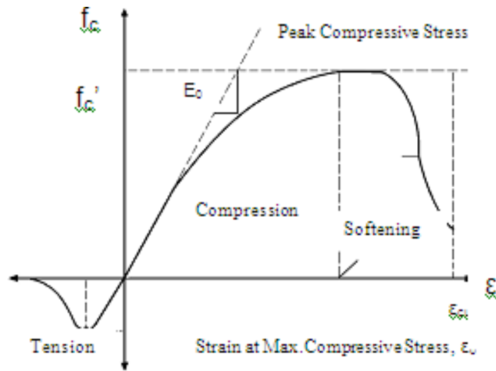
Fig -4: Stress –Strain Curve for Concrete
