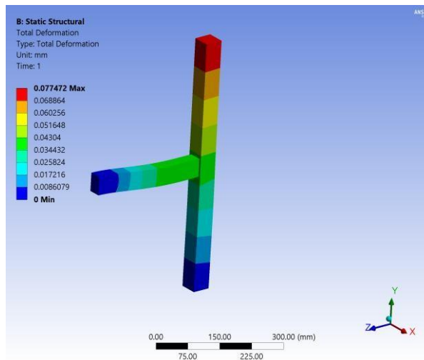
Fig -12: Total Deformation
