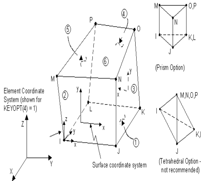
Fig -1: SOLID 45 Element
