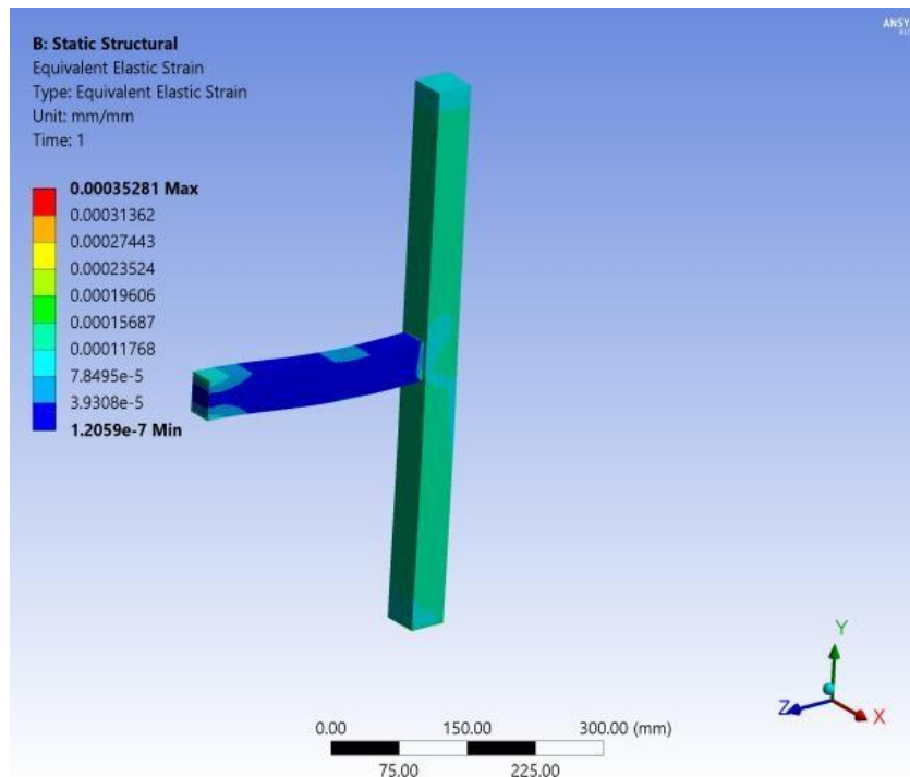
Fig -13: Equivalent Elastic Strain
