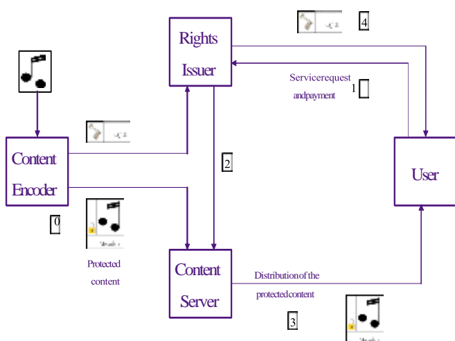
Figure 2: General architecture of a DRM system
