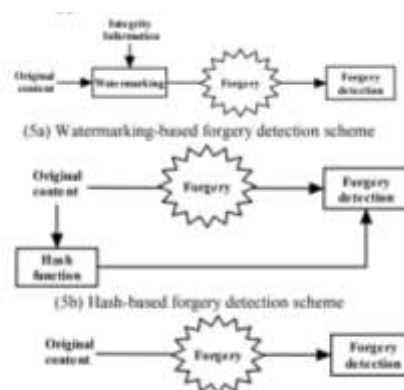
Figure 5: Various forgery detection schemes
