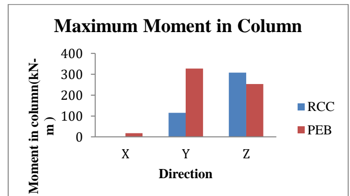
Fig. 6: Maximum Moments in Column
