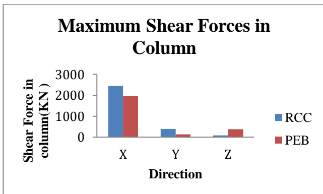
Fig. 5: Maximum shear forces in Column
