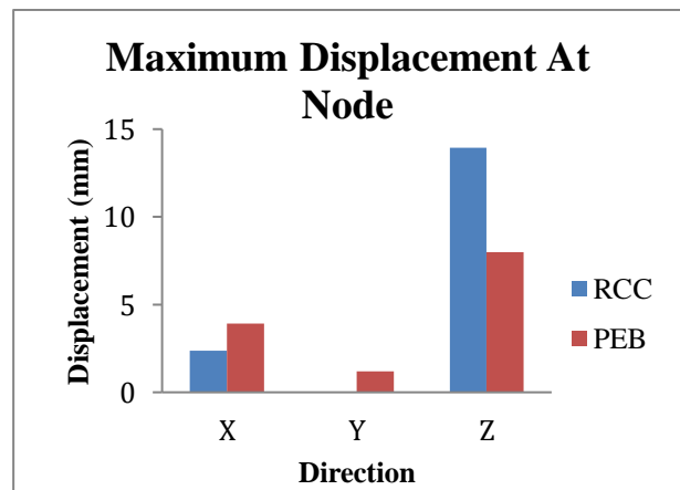
Fig. 3: Maximum displacements at node
