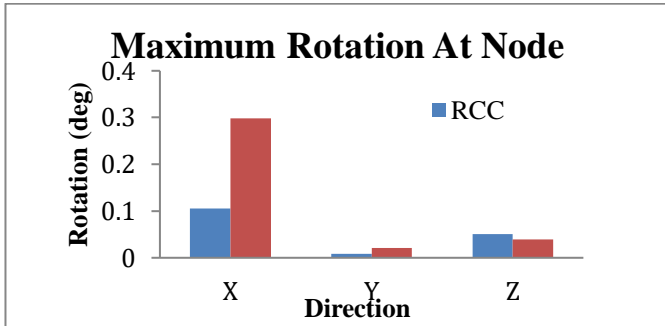
Fig. 4: Maximum Rotation at node
