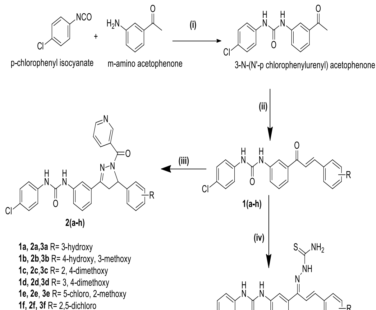
Fig.1g. The synthesis of the designed compounds 1a-1h, 2a-2h, 3a-3h (i) Me 2 CO, rt, 6 hr (ii) substituted benzaldehyde, methanolic NaOH, stirred at room temperature, 24 hr (iii) n-butanol, reflux (iv) thiosemicarbazide, EtOH, AcOH, reflux.
