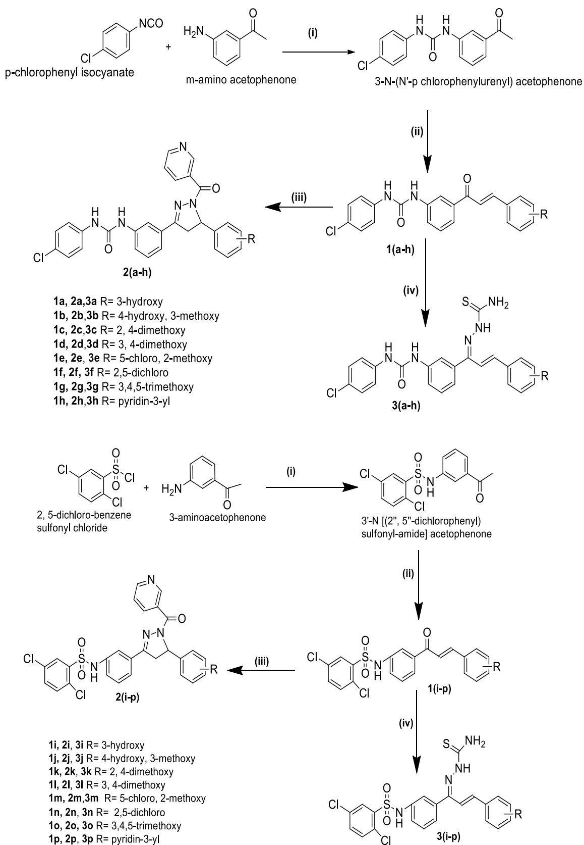
Fig. 6.1: The synthesis of the designed compounds 1a-1p, 2a-2p, 3a-3p
