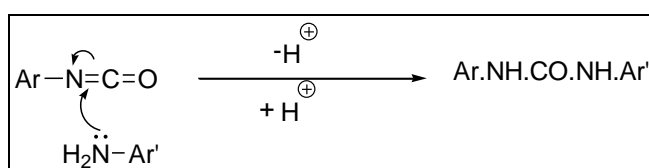
Figure : Scheme for synthesis of 3-N-(N'- p -chlorophenylurenyl)acetophenone
