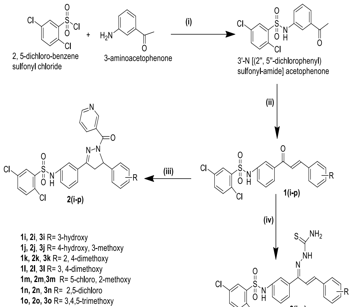
Fig. 1 The synthesis of the designed compounds 1i-1p, 2i-2p, 3i-3p (i) \text{CHCl}_3 , rt, 3-6 hrs (ii) substituted benzaldehyde, methanolic NaOH, stirred at room temperature, 24 hr (iii) n -butanol, reflux (iv) thiosemicarbazide, EtOH, AcOH, reflux.
