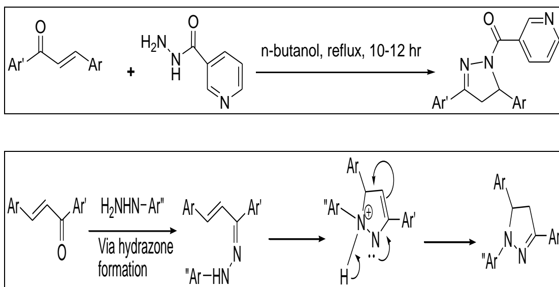
Figure : Scheme and mechanism of reaction for synthesis of compounds (2a-2p)
