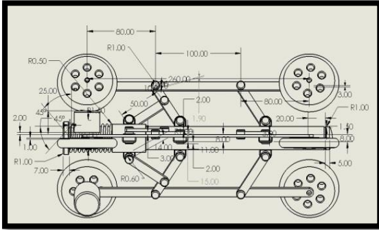
Fig. 1: Mechanism
