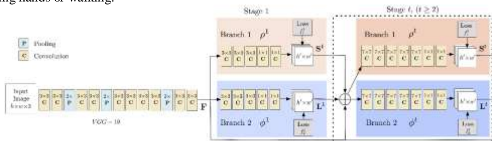
Fig. 1: OpenPose Architecture
