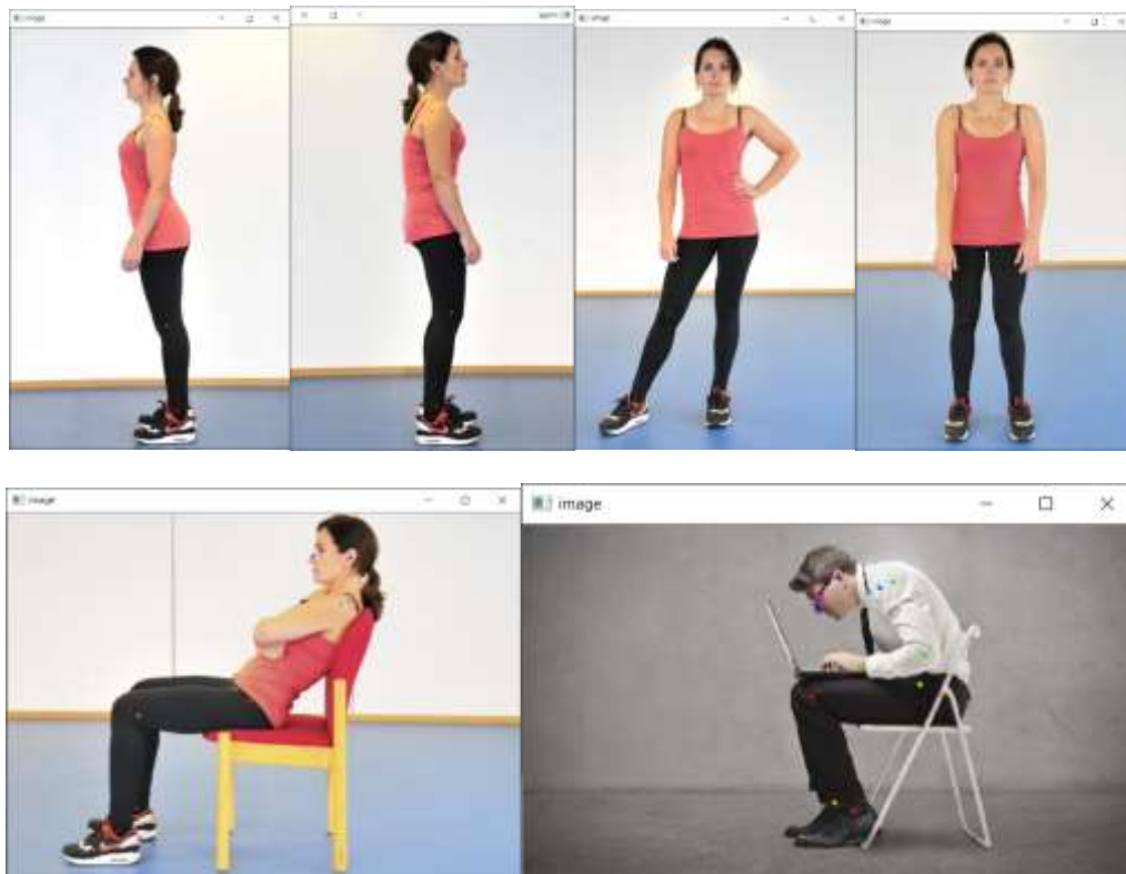
Fig. 3-10 The colour coded dot mapping after running the sample images through our model. The legs are colour coded to red and yellow the nose is colour coded to blue. The shoulder, elbow and wrist are green and eyes are pink.
