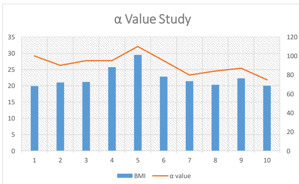
Fig. 11: \alpha value mapped against the BMI
