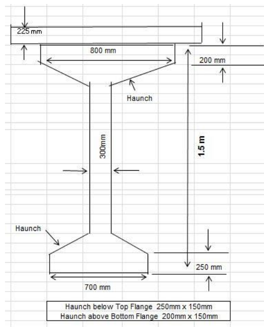
Figure: 4.0 – Cross Sectional Details of I Girder
