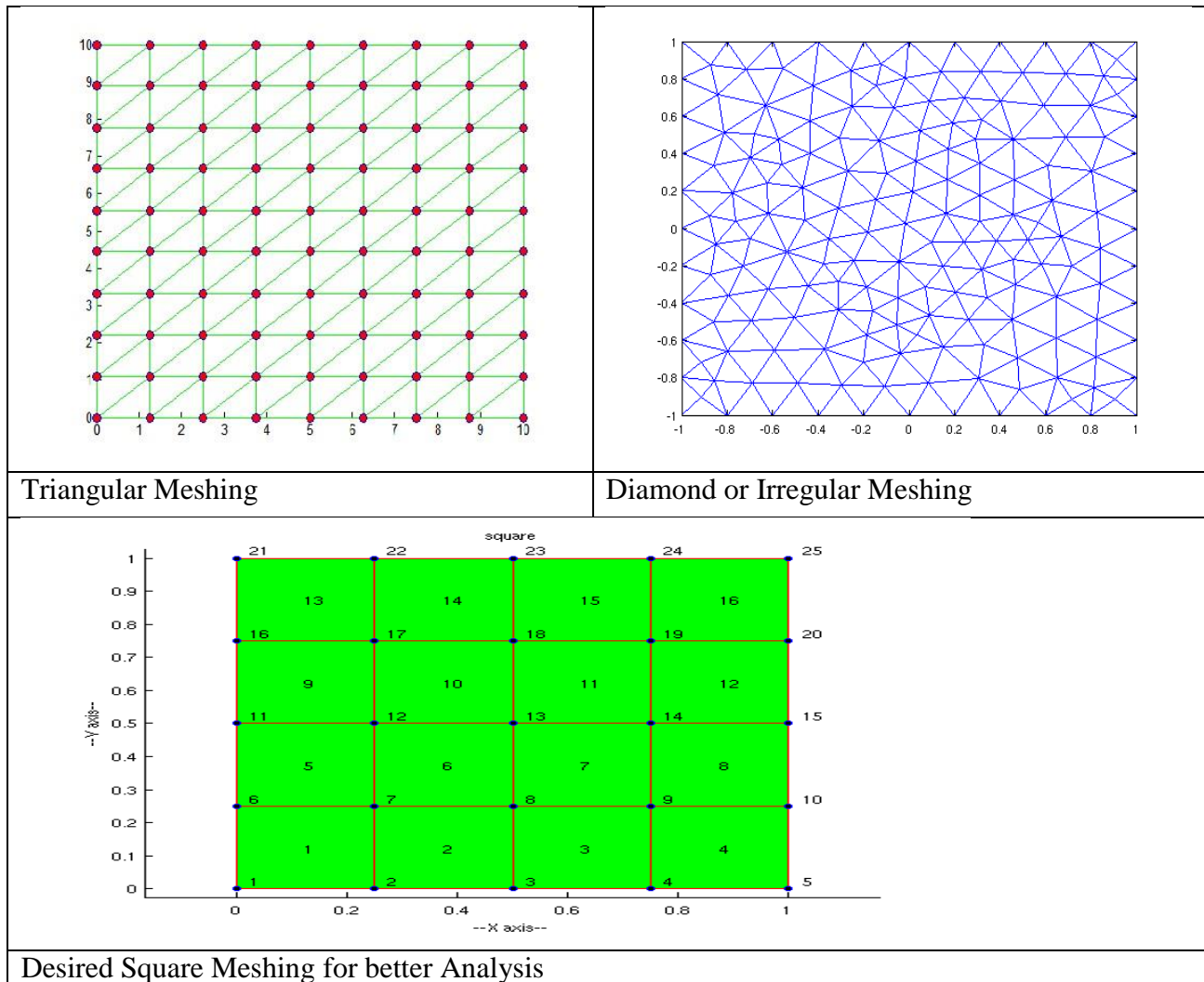
Figure: 1.0 – Different Types of Meshing Based on Shape
