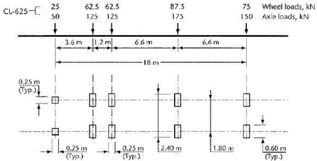
Figure: 9.0 – Axle Spacing and Load Distribution of CL-625 Truck Load
