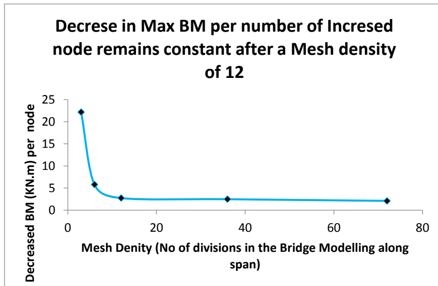
Figure: 11.0 – Variation of Decreased BM per Increase Node with Respect to Increase Mesh Density
