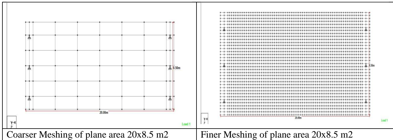
Figure: 2.0 – Coarser and Finer Meshing
