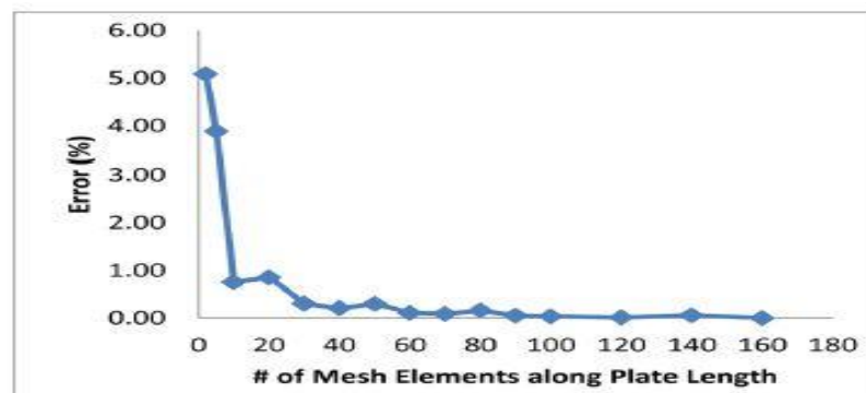
Figure: 3.0 – Variation of % of Error with Respect to Mesh Density (case study plot)
