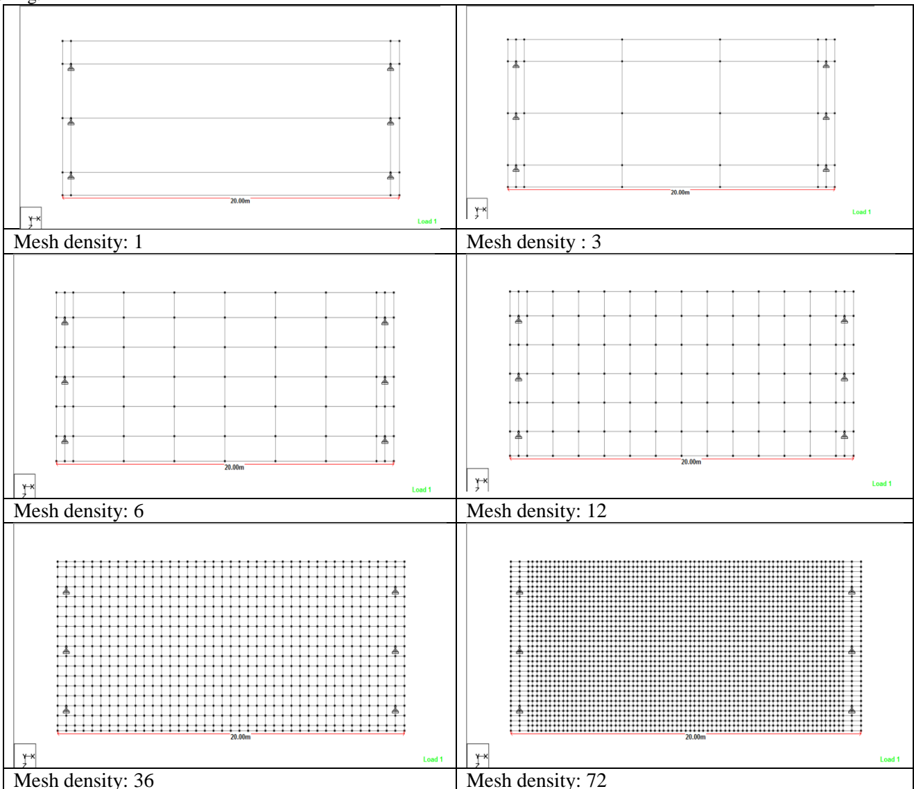
Figure: 6.0 – Modelling with Different Mesh Density
