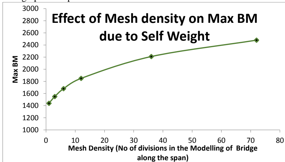
Figure: 7.0 – Variation of Max BM due to self-weight as per Mesh density
