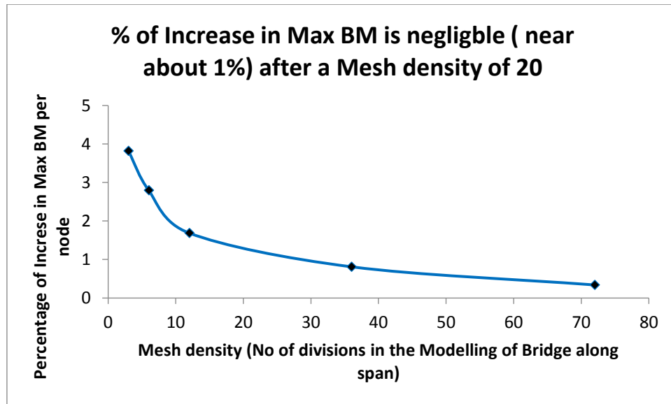
Figure: 8.0 – Variation in Percentage Increased of Max BM with Respect to Mesh Density
