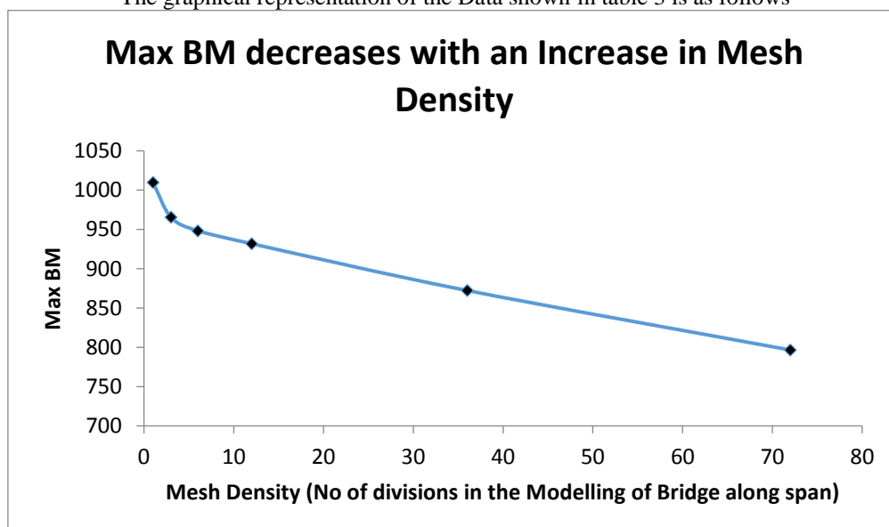
Figure 10.0 – Variation of Max BM due to living Load as per Increase in Mesh Density
