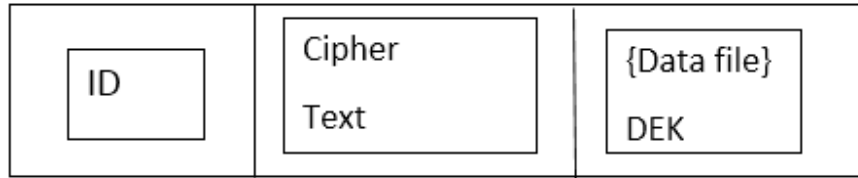
Fig 2. Format of Data on Cloud
