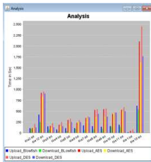
Fig 4. Comparison of Algorithms
