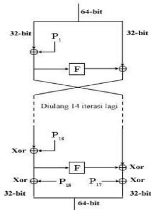
Fig 3. Blowfish Algorithm
