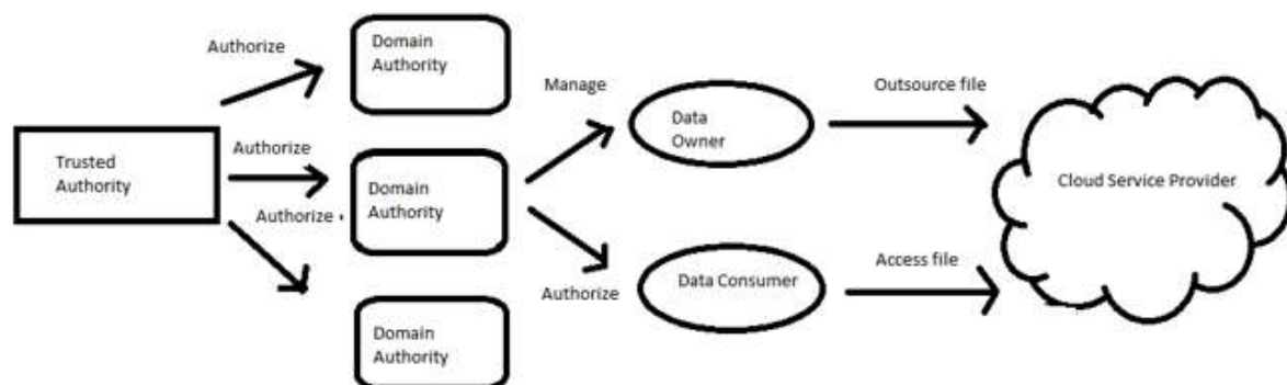
Fig 1. System Architecture
