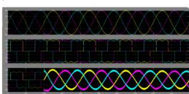
Fig 7 Voltage, distortion current waveform, after reducing current type harmonics
