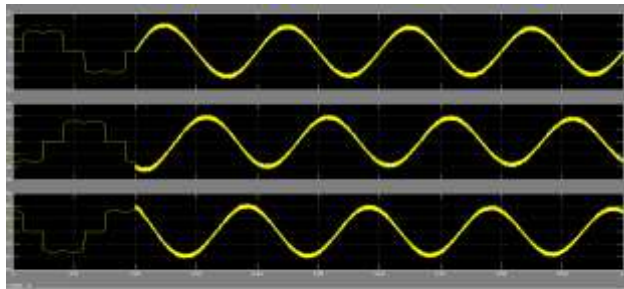
Fig 5 Output of three phase source after distortion and pure sine wave
