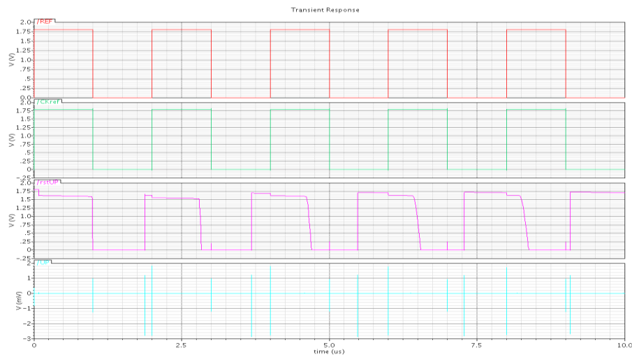
Fig. 8 Feedforward reset PFD transient response
