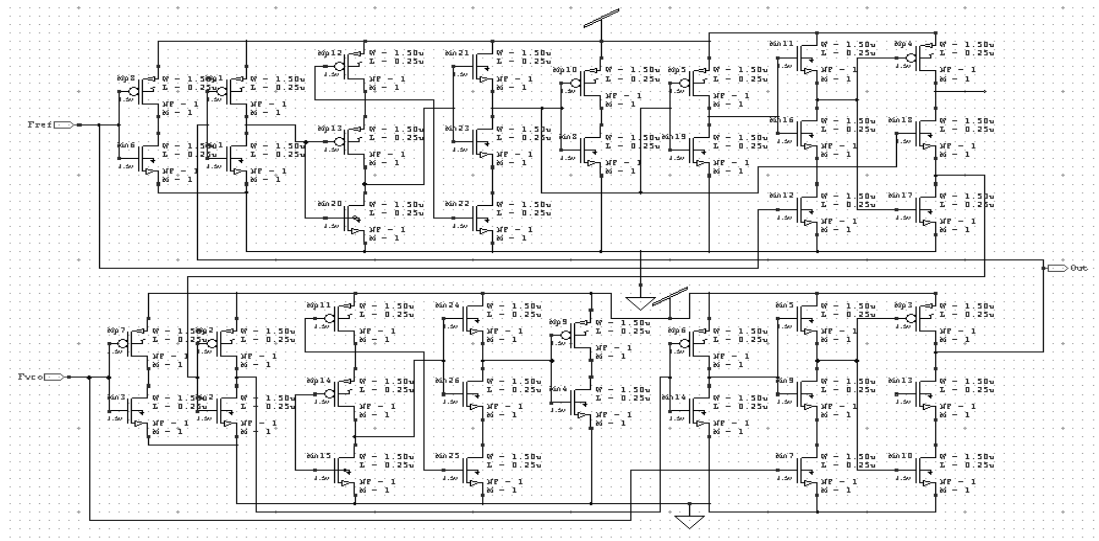
Fig. 7 Feedforward-Reset PFD
