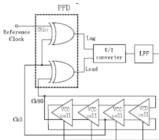
Fig. 3 PLL architecture [6]
