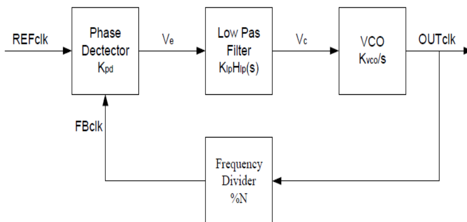
Fig. 1 Block diagram of PLL
