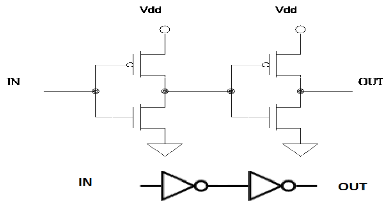
Fig. 5 Delay Cell
