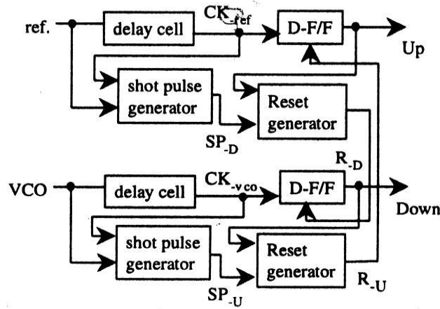
Fig. 4 Block diagram of feedforward-reset PFD
