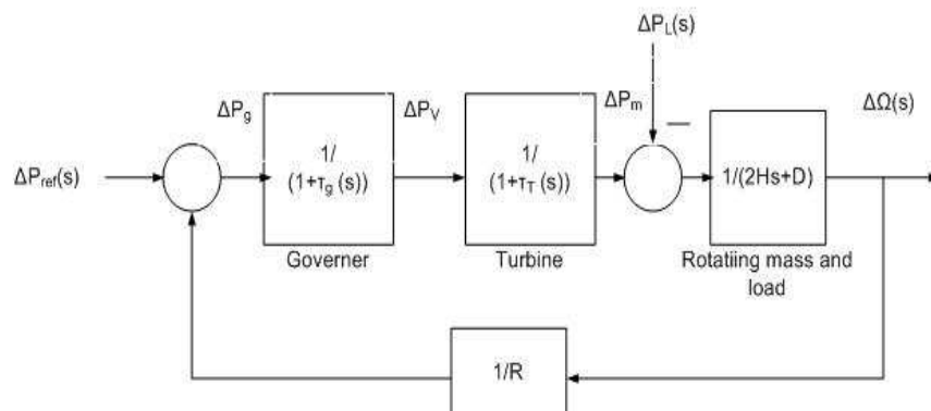
Fig 7: Block diagram of load frequency control of isolated power system
