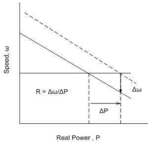
FIG.5: Governor speed characteristics
