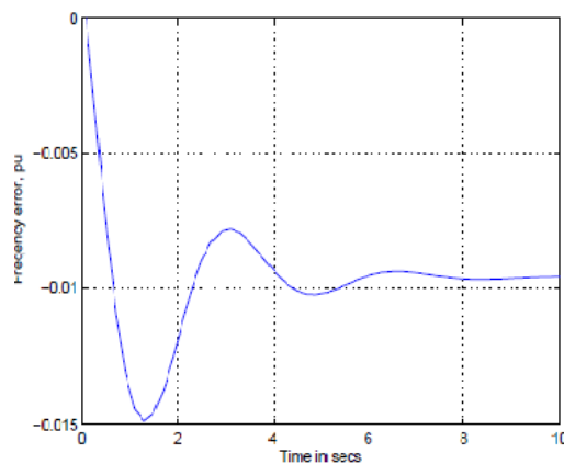
FIG. 8: Frequency deviation step response
