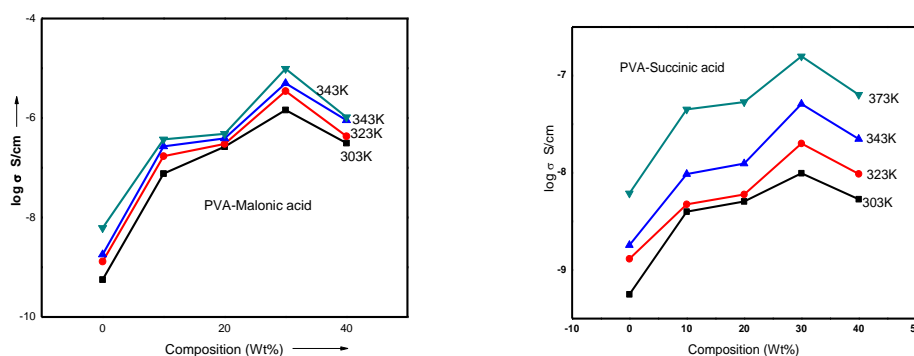
Fig.1 Composition vs conductivity of PVA: Malonic acid & PVA: Succinic acid polymer electrolytes with temperature as parameter.
