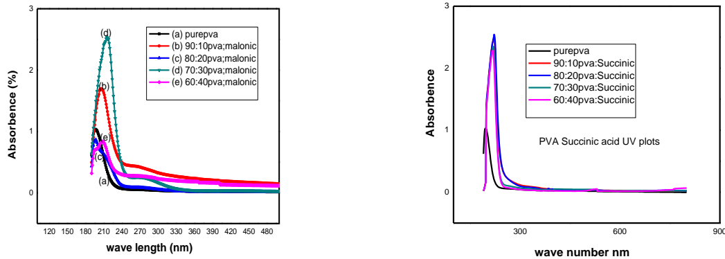
Fig.3 Optical absorption spectra of pure PVA and PVA doped Malonic & Succinic acid polymer electrolytes
