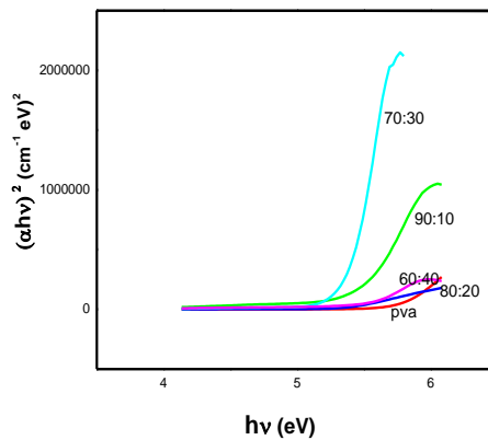
Fig.4 (a) (\alpha h\nu)^2 vs h\nu plots of pure and Malonic acid doped PVA polymer electrolytes
