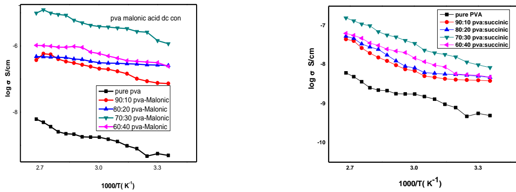
Fig.2 Conductivity log(σ) vs 1/T plots for PVA: Malonic acid & PVA: Succinic acid composite polymers
