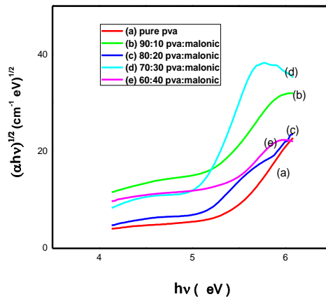
Fig.5(a). (\alpha hv)^{1/2} vs h\nu plots of pure and Malonic acid doped PVA polymer electrolytes.
