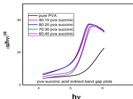
Fig.5 (b). (\alpha hv)^{1/2} vs h\nu plots of pure and Succinic acid doped PVA polymer electrolytes.
